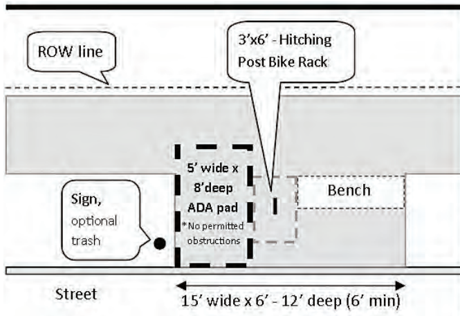
Figure 10 Type II Standard (Detached sidewalk)
