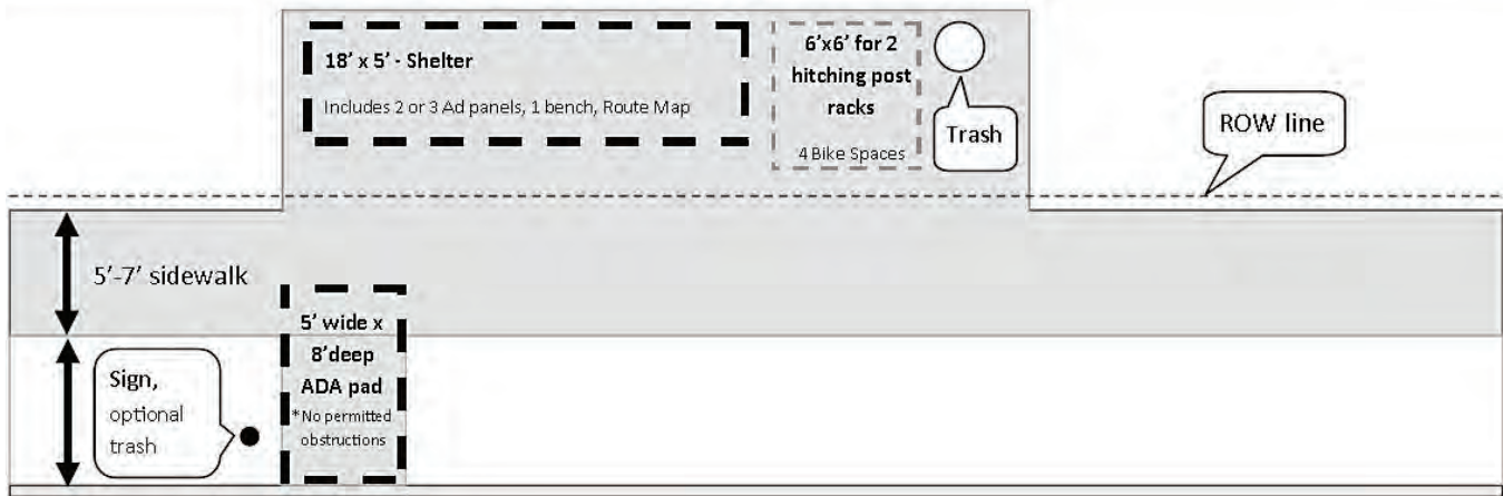
Figure 14 Type III Constrained (Detached sidewalk)
