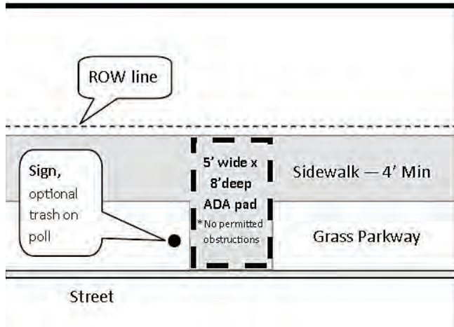
Figure 8 Type I Standard (Detached sidewalk)
