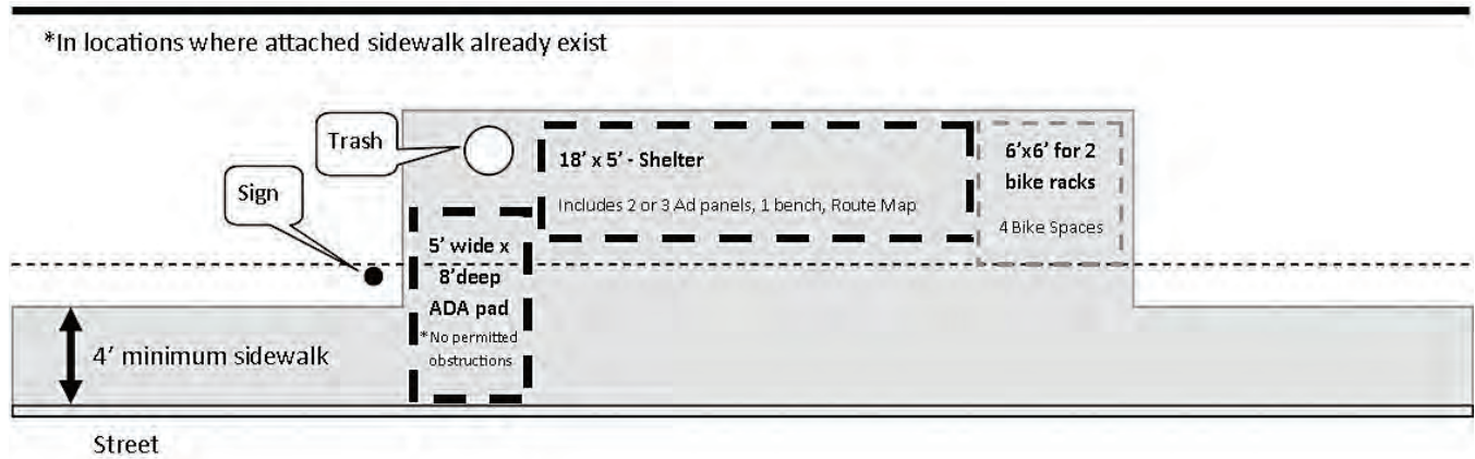
Figure 17 Type III Constrained (Attached sidewalk) – Amenity detail
