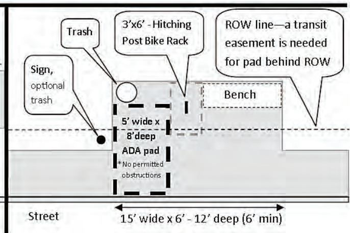
Figure 11 Type II Constrained (Attached sidewalk)
